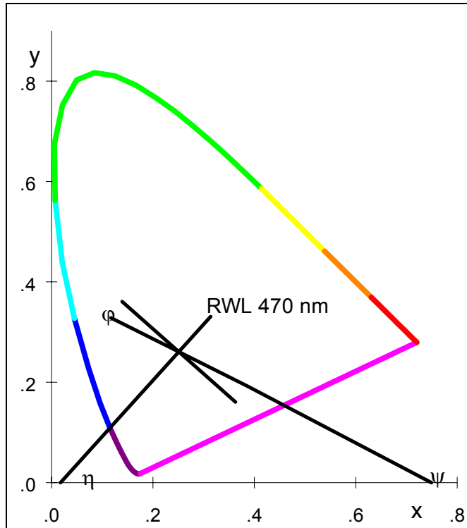
Fig. 1. Chromaticity chart D_{65}/10^\circ with RWL = 470 \text{ nm} , its perpendicular and the angles \varphi = 15^\circ and \psi = 153.18^\circ .
